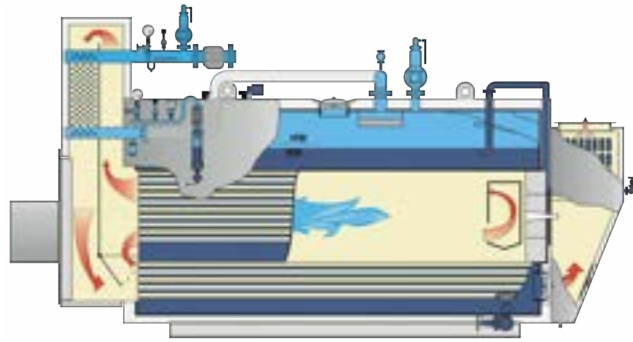
Sectional drawing UL-SX
